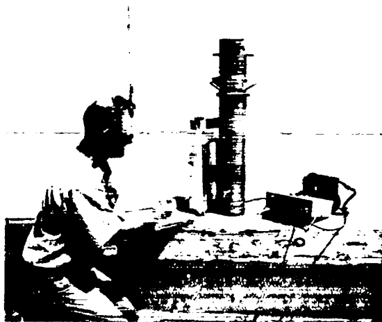
Fig. 28. Active neutron interrogation of a Type 5A container of \text{UF}_6 .
