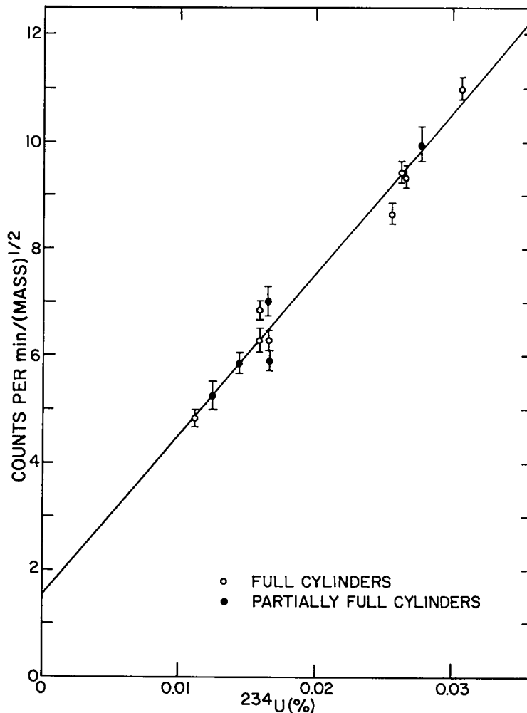
Fig. 27. Passive ^4\text{He} detector results.
