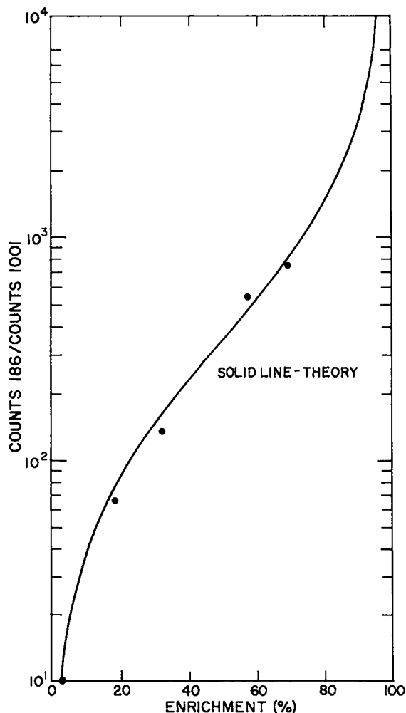
Fig. 21. Ratio of 186-keV to 1001-keV gamma rays for Type 1S UF 6 sample cylinders as a function of enrichment.
