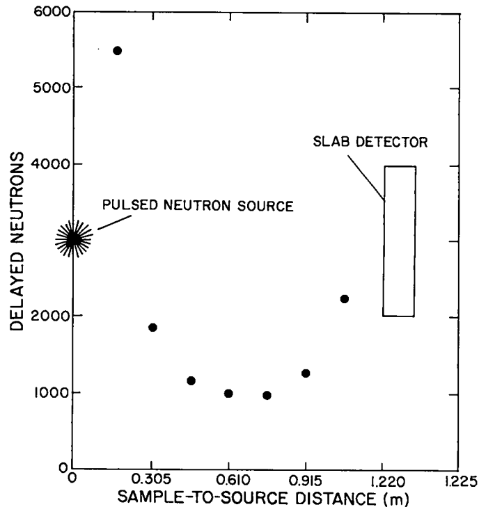
Fig. 15. Delayed fission neutrons detected for different package positions.
