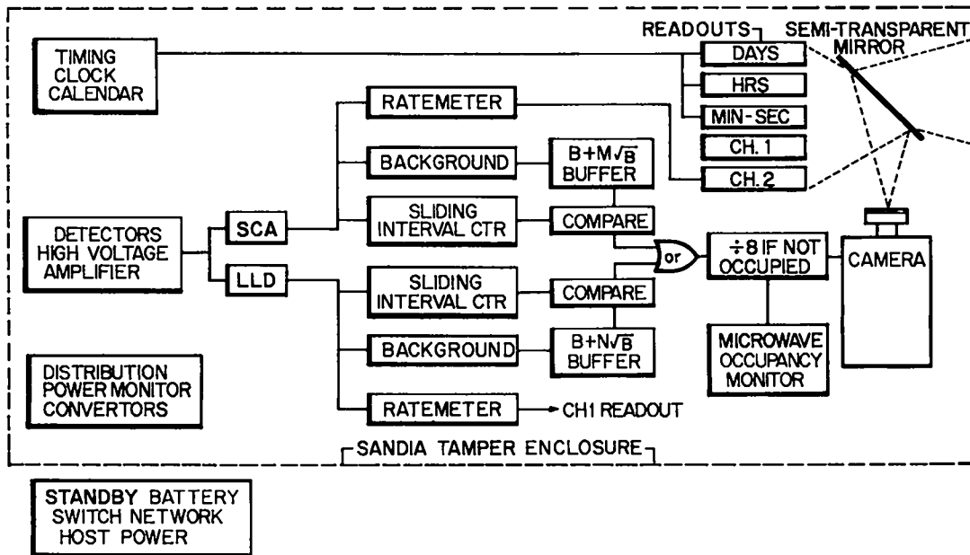
Fig. 6. Personnel doorway monitor: logic diagram.
