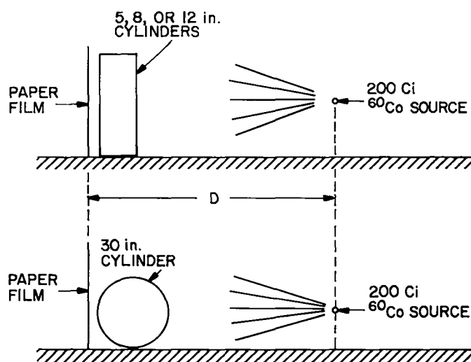
Fig. 30. Geometry used for cylinder radiography.
