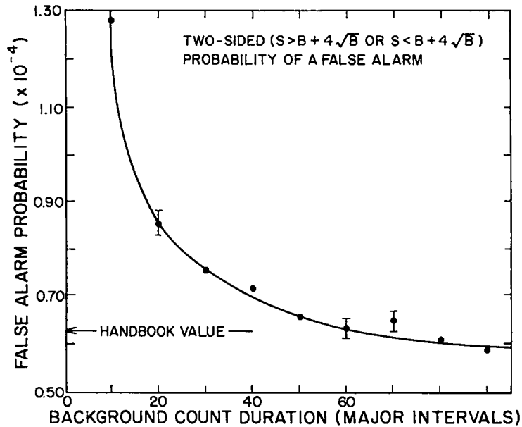
Fig. 9. Calculated false-alarm probability versus background count interval.
