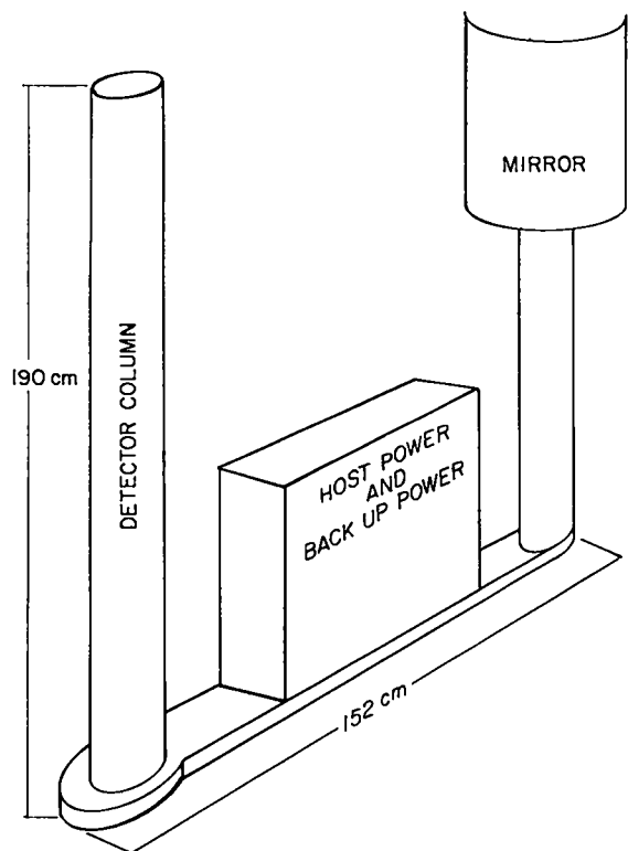
Fig. 13. Shipping dock monitor.
