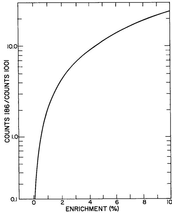
Fig. 20. Ratio of 186-keV to 1001-keV gamma-ray counts as a function of enrichment for Type 5A cylinders using a small NaI detector.
