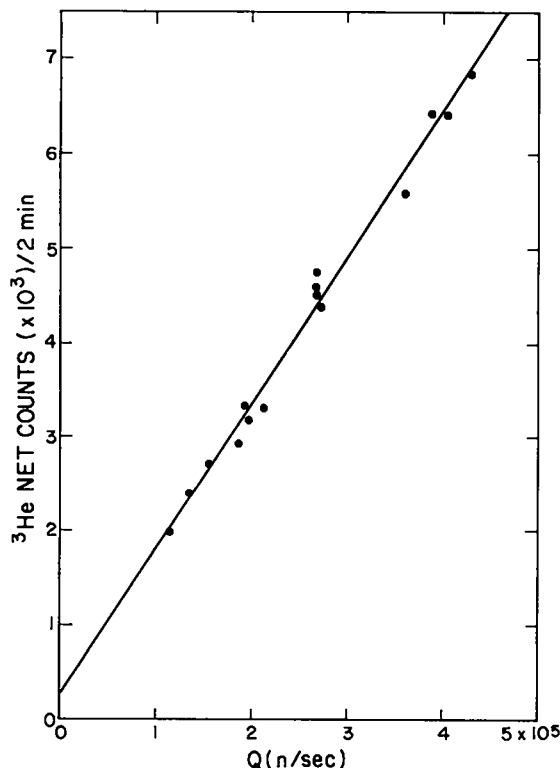
Fig. 25. Measured neutron count rate compared to the neutron source strength calculated in Case 1.
