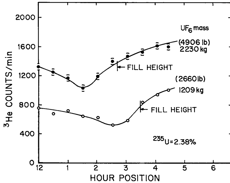
Fig. 24. ^3\text{He} detector circumferential scan of Type 30A cylinders of identical enrichment but different fill levels.
